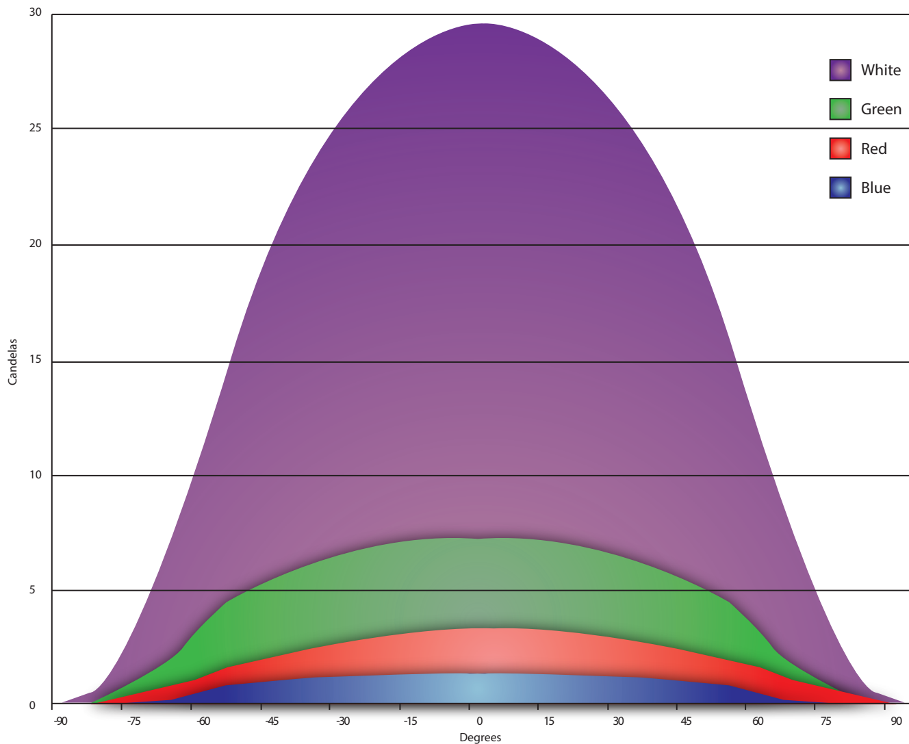
4x1 Trilite RGBW Photometric Sweep
