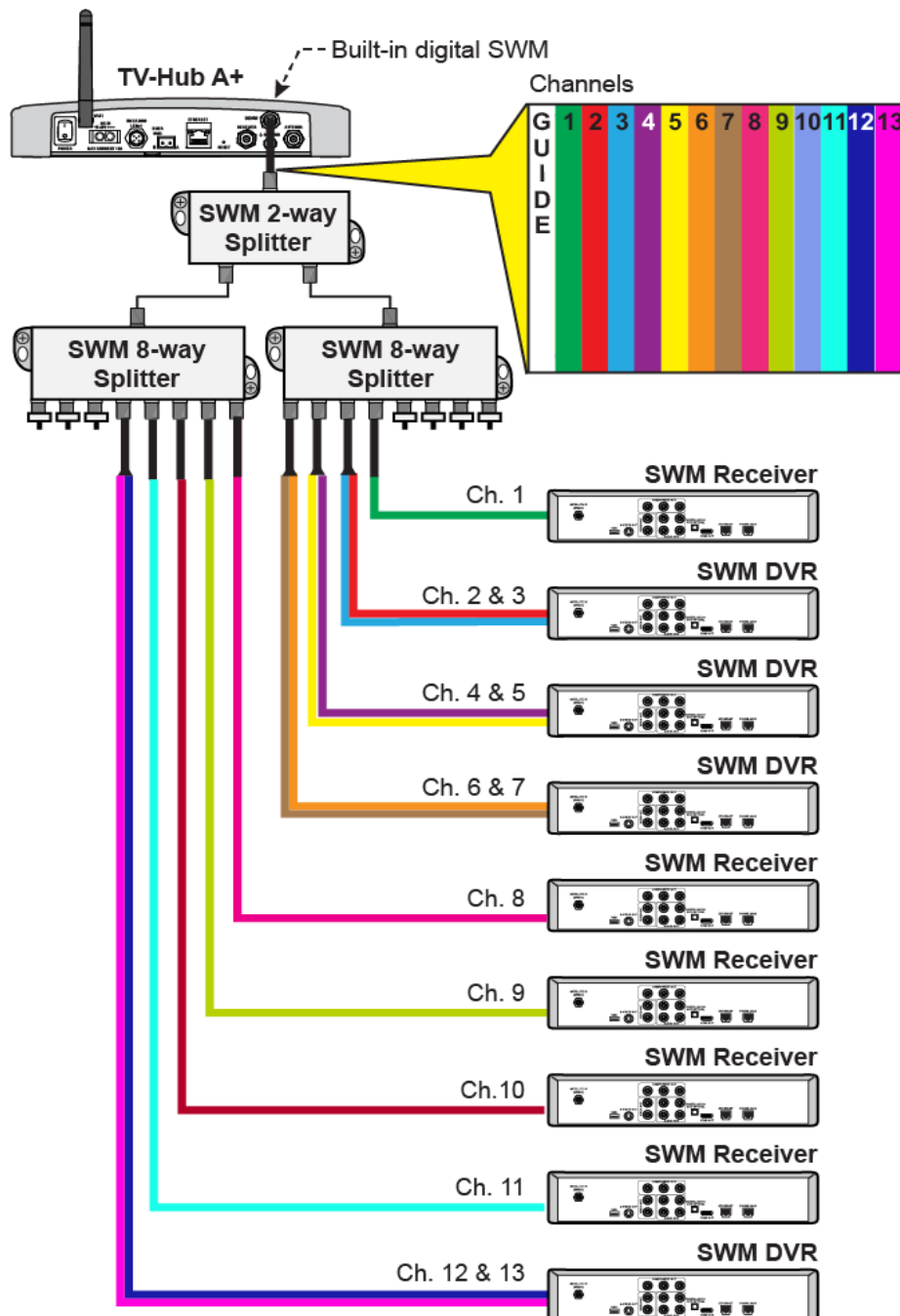
Figure 7-6 DIRECTV SWM Technology (TV-Hub A+)
