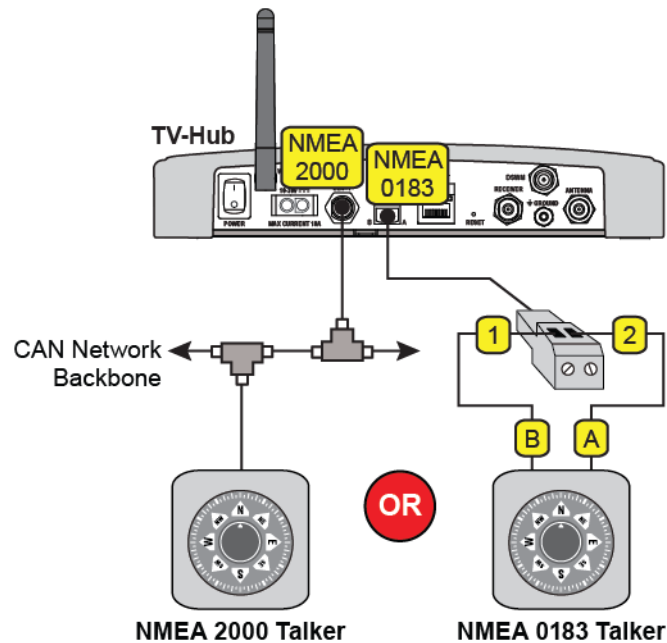
Figure 4-1 TV-Hub NMEA Connections (TV-Hub A+ shown)
