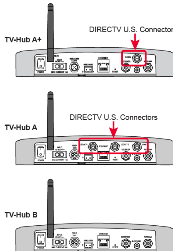
Figure 1-4 TV-Hub Versions
