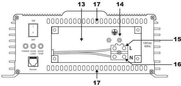
PST-1500 & PST-2000: FRONT - showing compartment containing AC output terminals for hardwiring.
